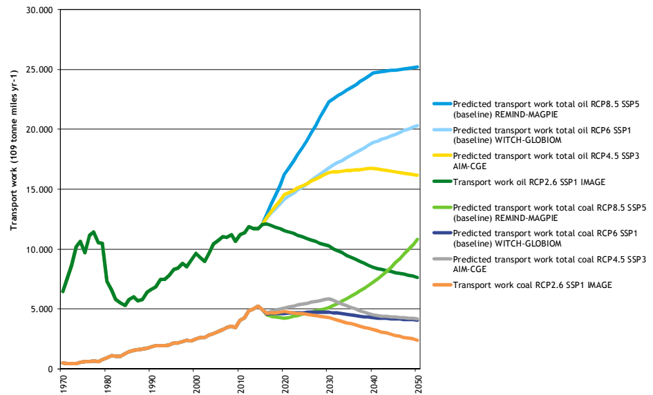
Historical and predicted coal and oil shipping according to RCPs
