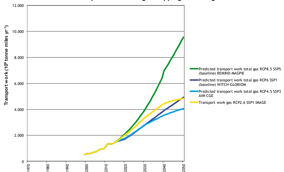
Historical and predicted total gas shipping according to RCPs
