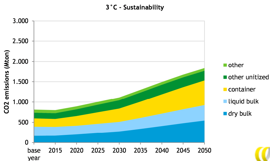
Figure 15 CO 2 emission projections of different ship types in the 3°C - sustainability scenario
