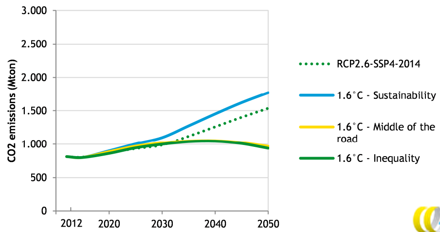
Figure 1 CO 2 emission projections of shipping in three 1.6°C scenarios
