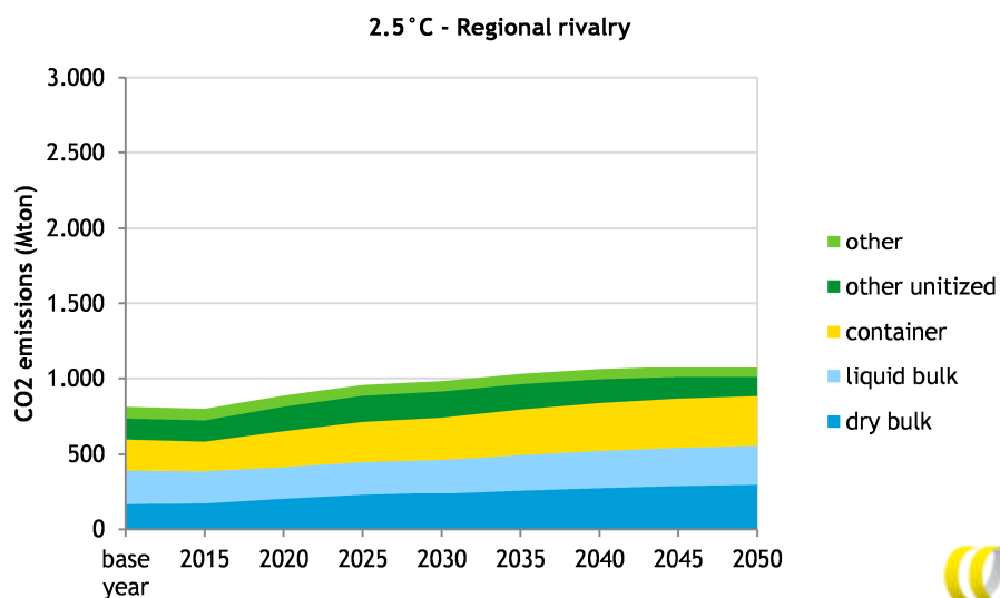
Figure 14 CO 2 emission projections of different ship types in the 2.5°C - regional rivalry scenario
