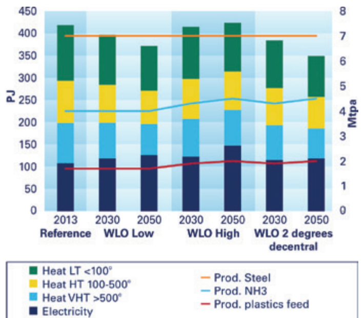
Figure 2. Development of energy use in industry in WLO scenarios
