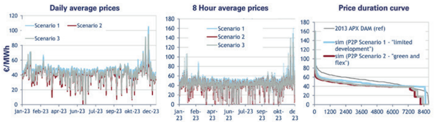
Figure 5. Volatility depicted in price levels on different time scales (2023) (€ 2015 /MWh) Source: (Berenschot, CE Delft, ISPT, 2015)
