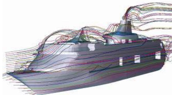
Figure A2-3 – A CFD analysis of wind resistance (CFD Norway)
