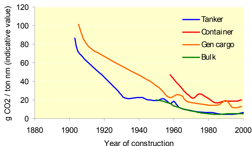
Figure 9-5 – Indicative development in maximum ship design transport efficiency
