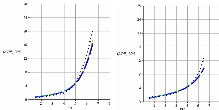
Figure A3-2 – Speed loss (drop) of a ship in irregular head waves and wind (waves and wind from the same direction 180°) – comparison between the approximate formulae and detailed calculations for (a) Large tanker (loaded and/or normal condition), displacement volume \nabla = 350,000 \text{ m}^3 , Fn = 0.15 , C_B = 0.84 , L_{pp} = 336.0 \text{ m} ; (b) Large containership (loaded and/or normal condition), displacement volume \nabla = 60,200 \text{ m}^3 , Fn = 0.25 , C_B = 0.62
