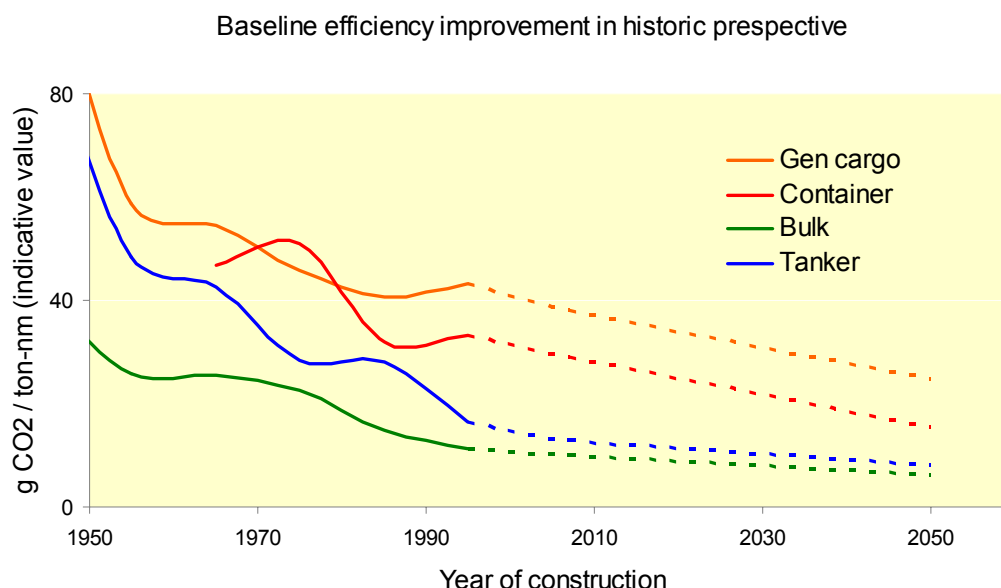
Figure 7-3 – Baseline improvements in efficiency and indicated historic improvements
