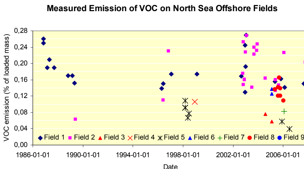
Figure 3-5 – VOC emission factor measured during offshore loading in the North Sea
