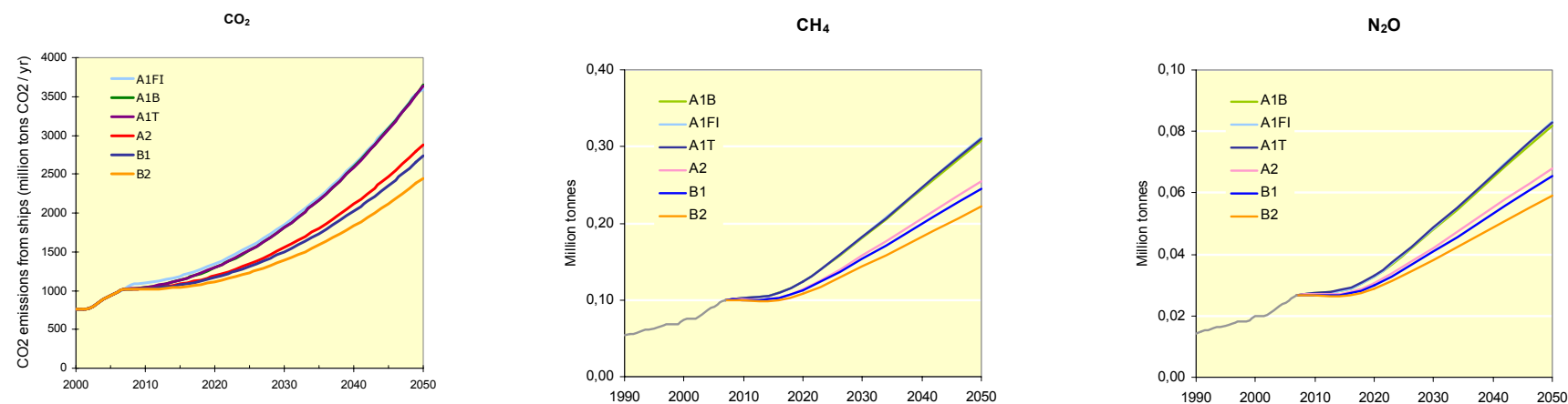
Figure 7-8 – Emission scenario trajectories for GHG emissions – total shipping (exhaust emissions only)
