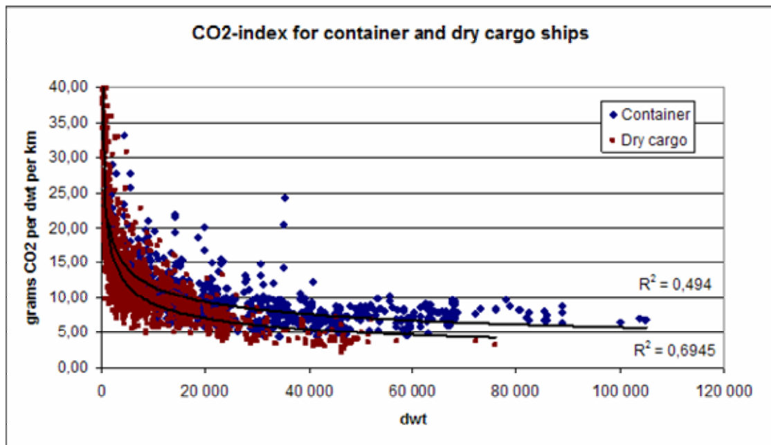
Figure 6-1 – The effect of ship deadweight on CO 2 design index [2]
