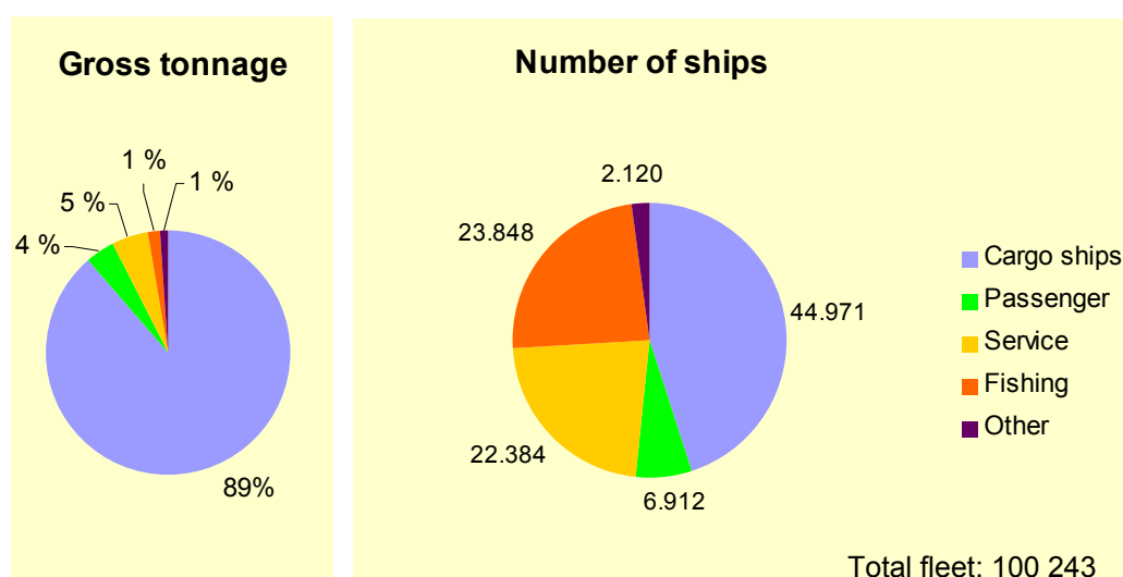
Figure 2-5 – Composition of the world fleet [Lloyd's Register – Fairplay, 2007]
