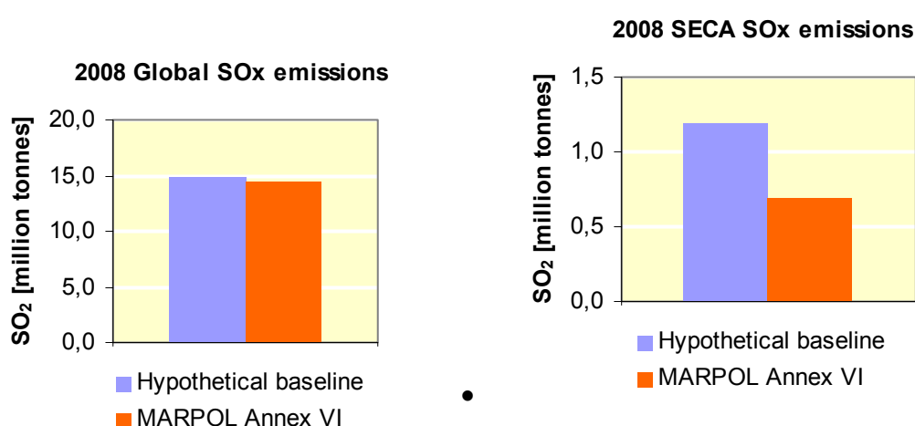
Figure 4-4 – Reductions of emissions of SO x estimated for 2008
