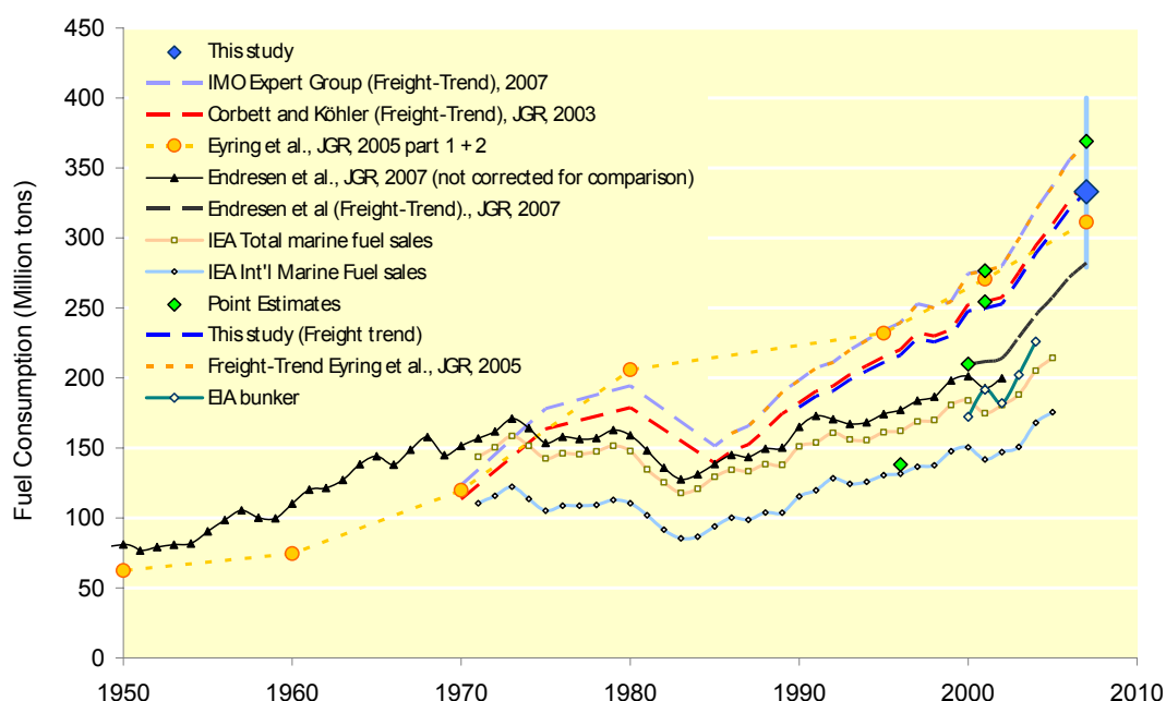
Figure 3-2 – World fleet fuel consumption (except military vessels) from different activity-based estimates and statistics. Symbols indicate the original estimates for individual years and the solid lines show the original estimates of trend. Dashed lines show the backcast and forecast, calculated from the time evolution of freight tonne-miles with the point estimates. The blue square shows the activity-based estimate from this study and the blue range bar indicates the high and low bound estimates
