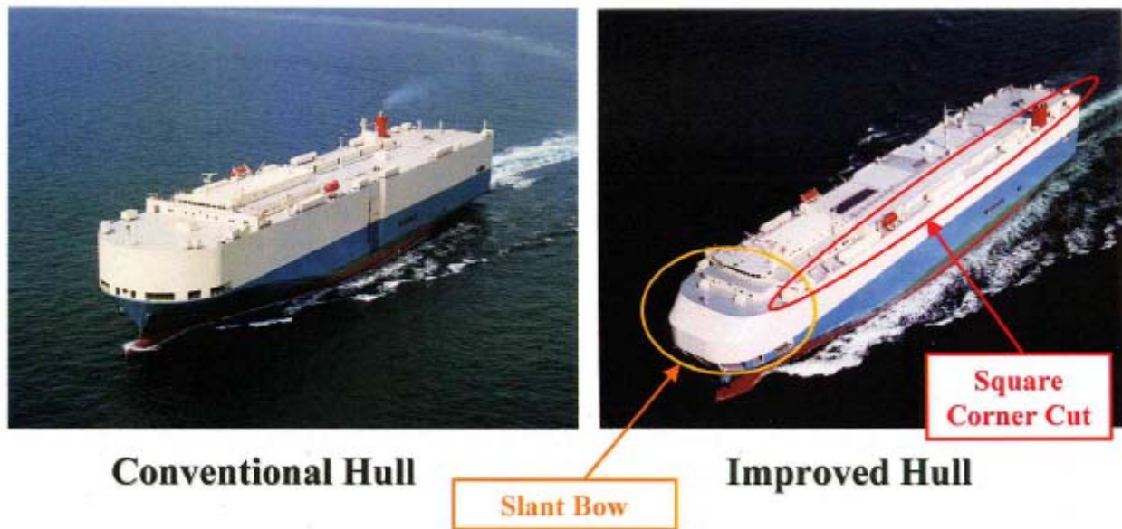
Figure A2-4 – Example of improvements to a superstructure (Universal Shipbuilding)
