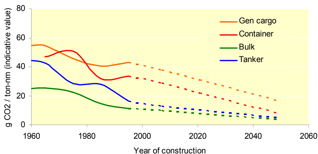
Figure 5-1 – Indicated historical efficiency and “high-efficiency” scenarios
