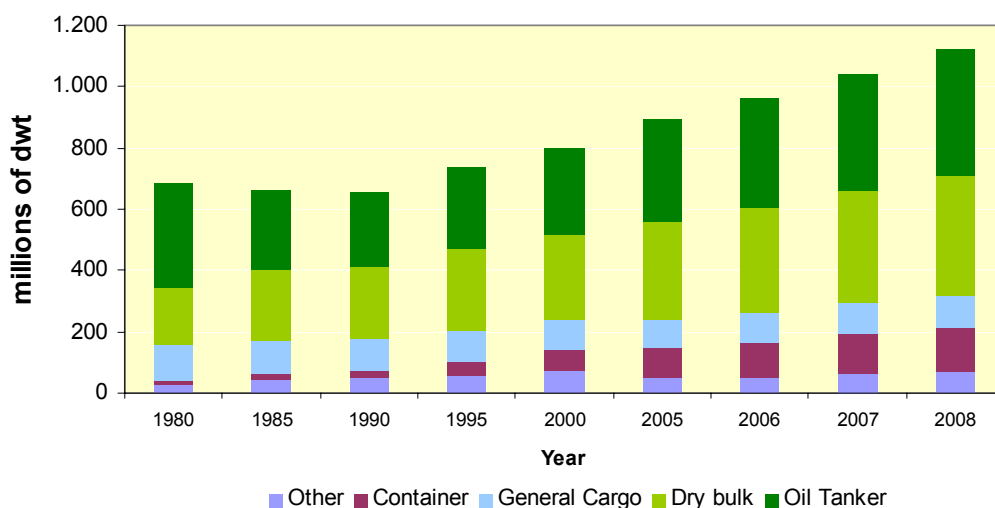
Figure 2-7 – Fleet growth in millions of dwt per major ship type, 1980 to 2008 [UNCTAD, 2008]
