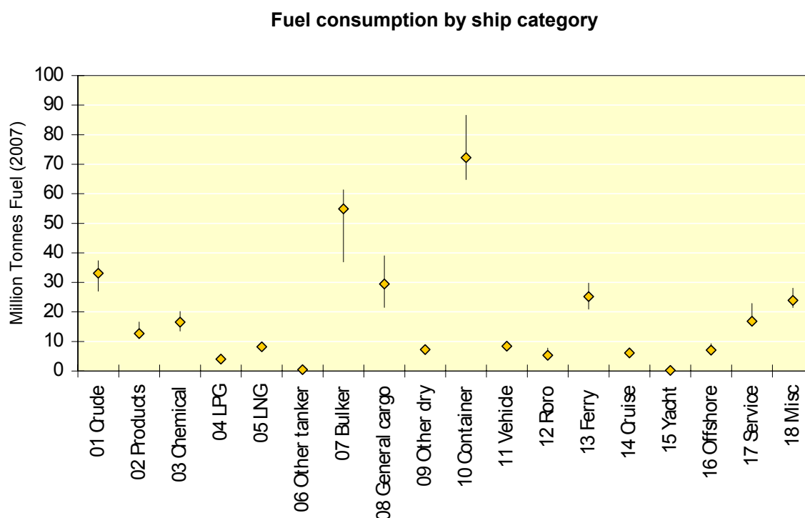
Figure A1-6 – Estimated fuel consumption (million tonnes) in 2007 by main ship categories, with uncertainty bars
