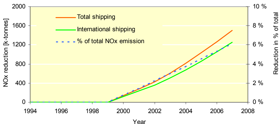
Figure 4-3 – NO x reductions achieved by regulation 13
