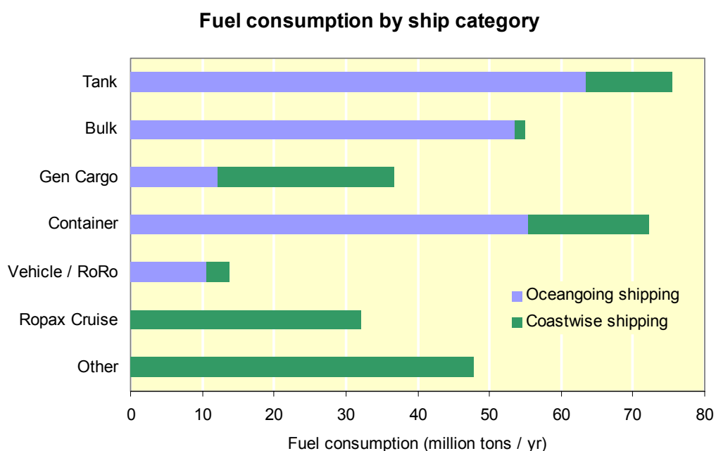
Figure 3-3 – Fuel consumption, separated into consumption by main categories of vessel and assumed typical types of operation (Coastwise shipping is mainly ships < 15 000 dwt, RoPax, Cruise, Service and Fishing)
