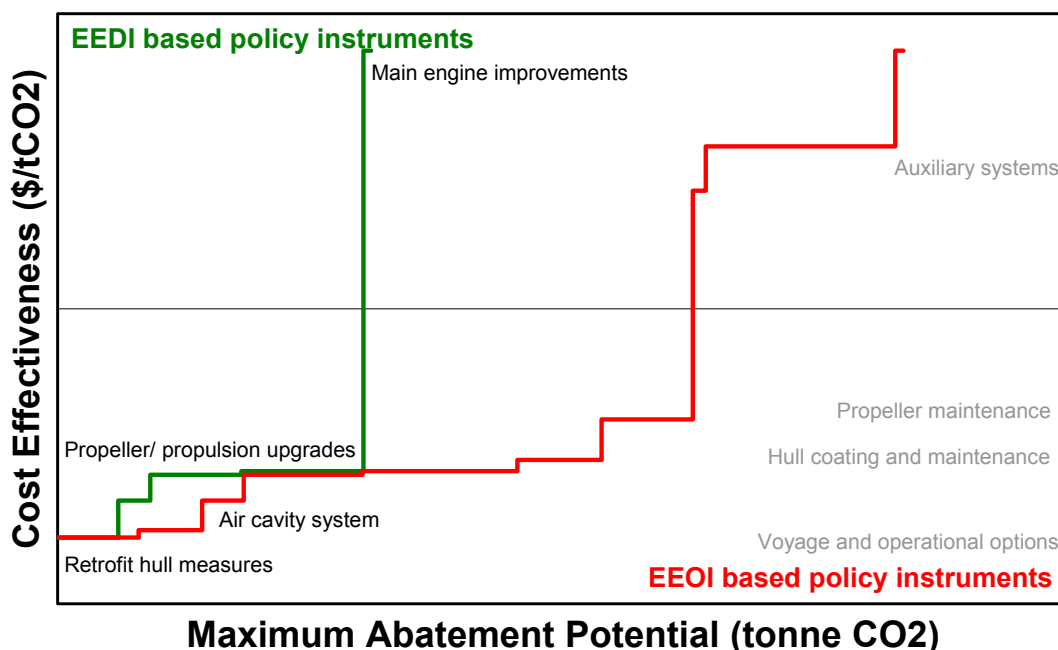
Figure 6-3 – Marginal abatement cost curves for 2020, with fuel at US$500 per tonne
