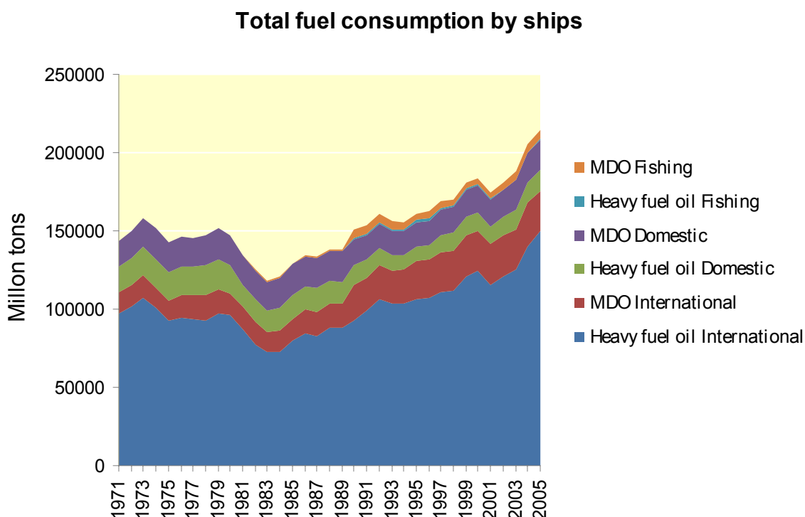
Figure A1-3 – Total fuel consumption by ships (Figure based on IEA data)
