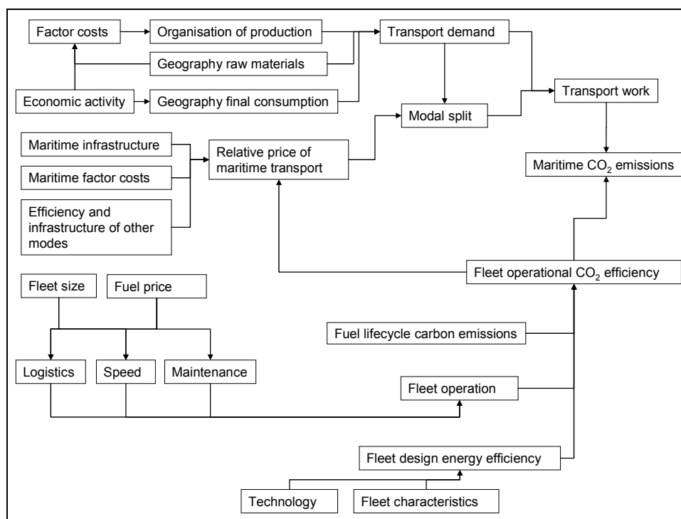
Figure 6-2 – Stylized representation of factors determining maritime emissions
