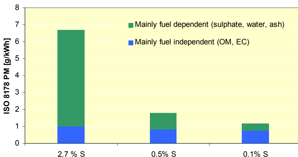
Figure A2-7 – The influence of fuel on PM mass. Data: GL [7]
