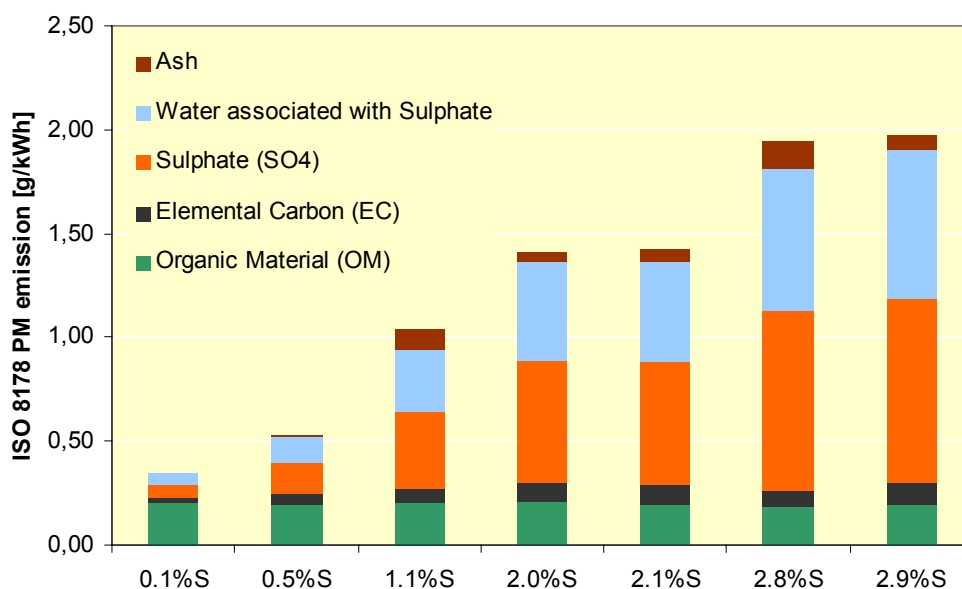
Figure 7-6 – The compositions of particulate matter obtained from different fuel types, Germanischer Lloyd [24]
