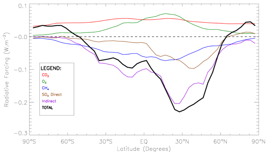
Figure 8-6 – Zonal mean annual RF pattern from shipping for the IMO estimates of RF in 2007 (modified from Lee et al. , 2009a).
