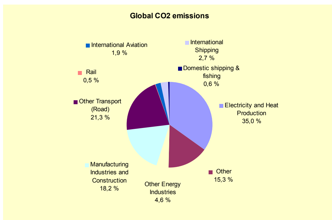
Figure 9-7 – Emissions of CO 2 from shipping compared with global total emissions
