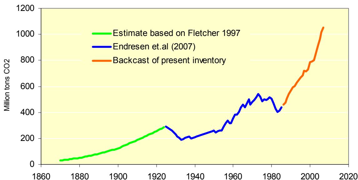
Figure 8-2 – Historical and present-day emissions of CO 2 from shipping
