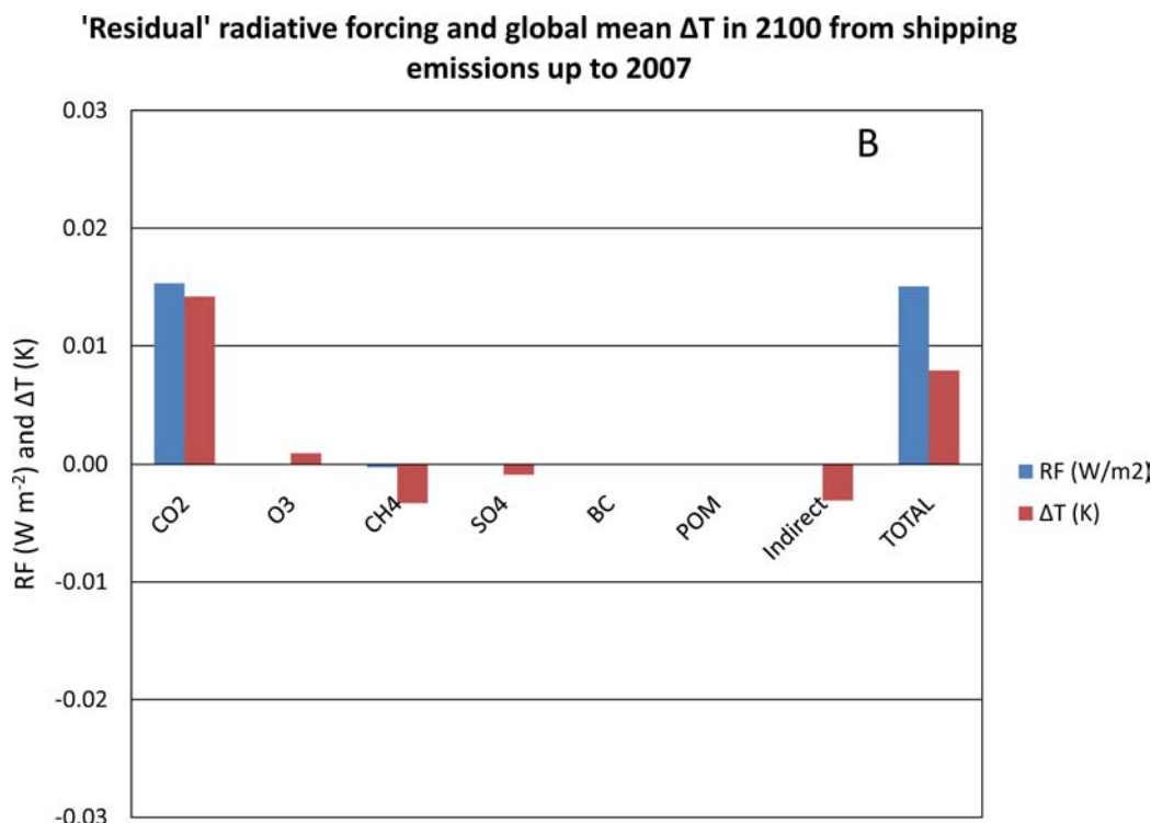
Figure 8-5 –Residual radiative forcing and temperature responses from shipping emissions to 2007 in 2050 (panel A) and 2100 (panel B). The figure does not include the positive RF that could potentially occur from the interaction of BC with snow that has, so far, not been investigated for ships.
