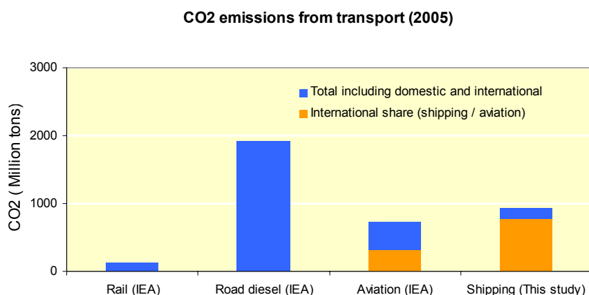
Figure 9-6 – Emissions of CO 2 in 2005 from shipping compared to other transport modes
