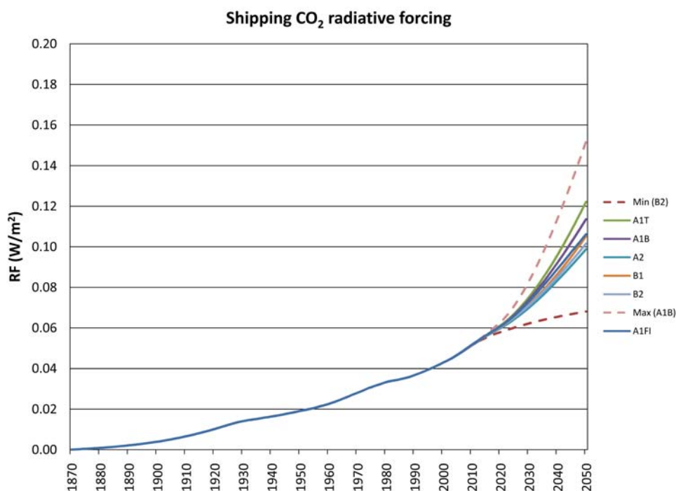
Figure 8-3 – Radiative forcing of CO 2 attributable to shipping from 1870 to 2005, and thereafter, according to a range of scenarios, to 2050
