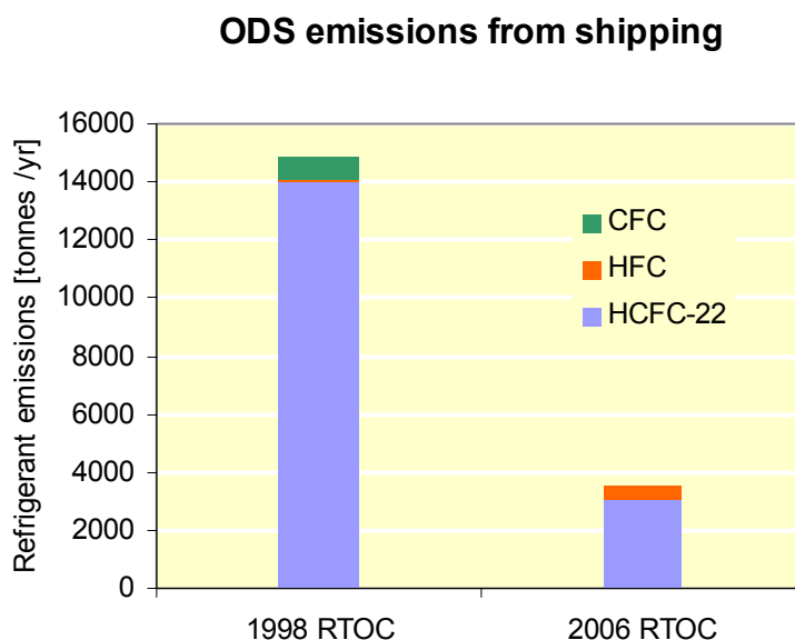
Figure 4-1 – Estimated emissions of ozone-depleting substances [UNEP]
