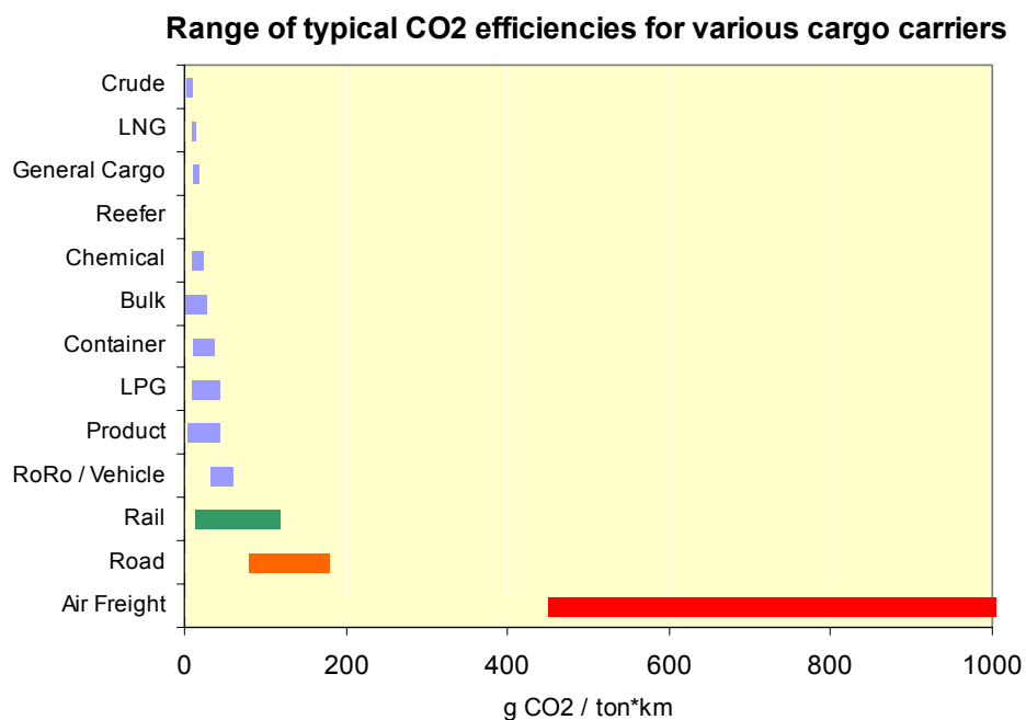
Figure 9-3 –Typical range of ship CO 2 efficiencies compared to rail, road and airfreight
