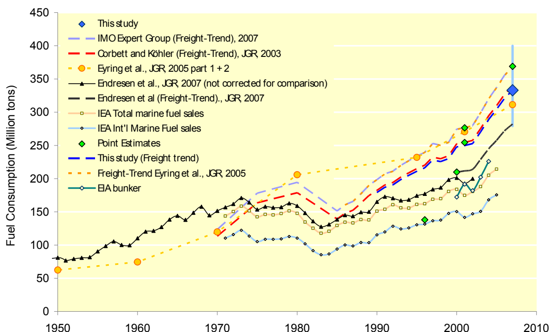
Figure A1-4 – World fleet fuel consumption (except naval vessels) from different activity-based estimates and statistics. Symbols indicate the original estimates for individual years and the solid lines show the original estimates of trend. Dashed lines show the backcast and forecast, calculated from the time evolution of freight tonne-miles with the point estimates. The blue square shows the activity-based estimate from this study and the blue range bar indicates the high and low bound estimates
