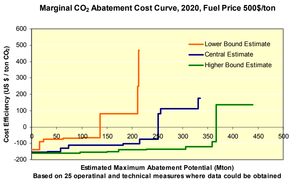
Figure 5-2 – Indicative marginal CO 2 abatement costs for 2020
