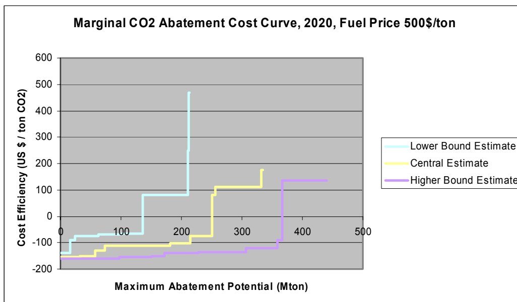
Figure A4-1 – Marginal CO 2 abatement cost curve for 2020, a fuel price of US$500/tonne and an interest rate of 4%
