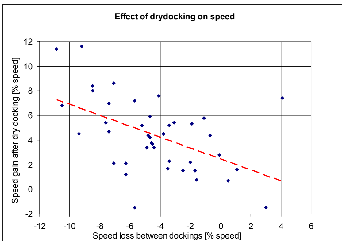
Figure A2-5 – The effect of dry-docking on the speed of a tank ship; the analysis is based on data reported by the ship (Primarily, TBT-based self-polishing coatings were used)
