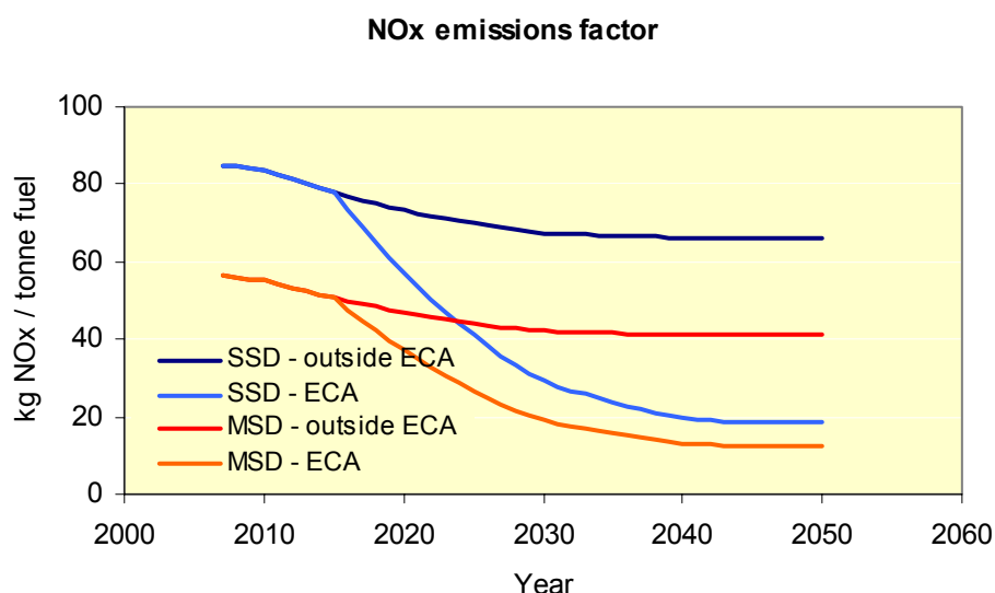
Figure 7-4 – Future NO x emission factors (3% fleet growth per year, 30 year vessel life)
