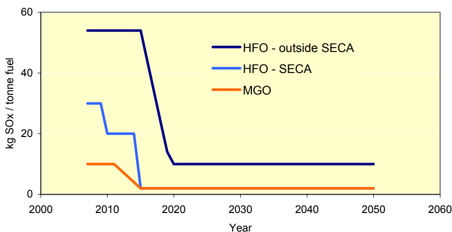
Figure 7-5 – Future SO x emission factors used in scenarios. The limit of 3.5% on global sulphur content is not expected to influence the average emission factor
