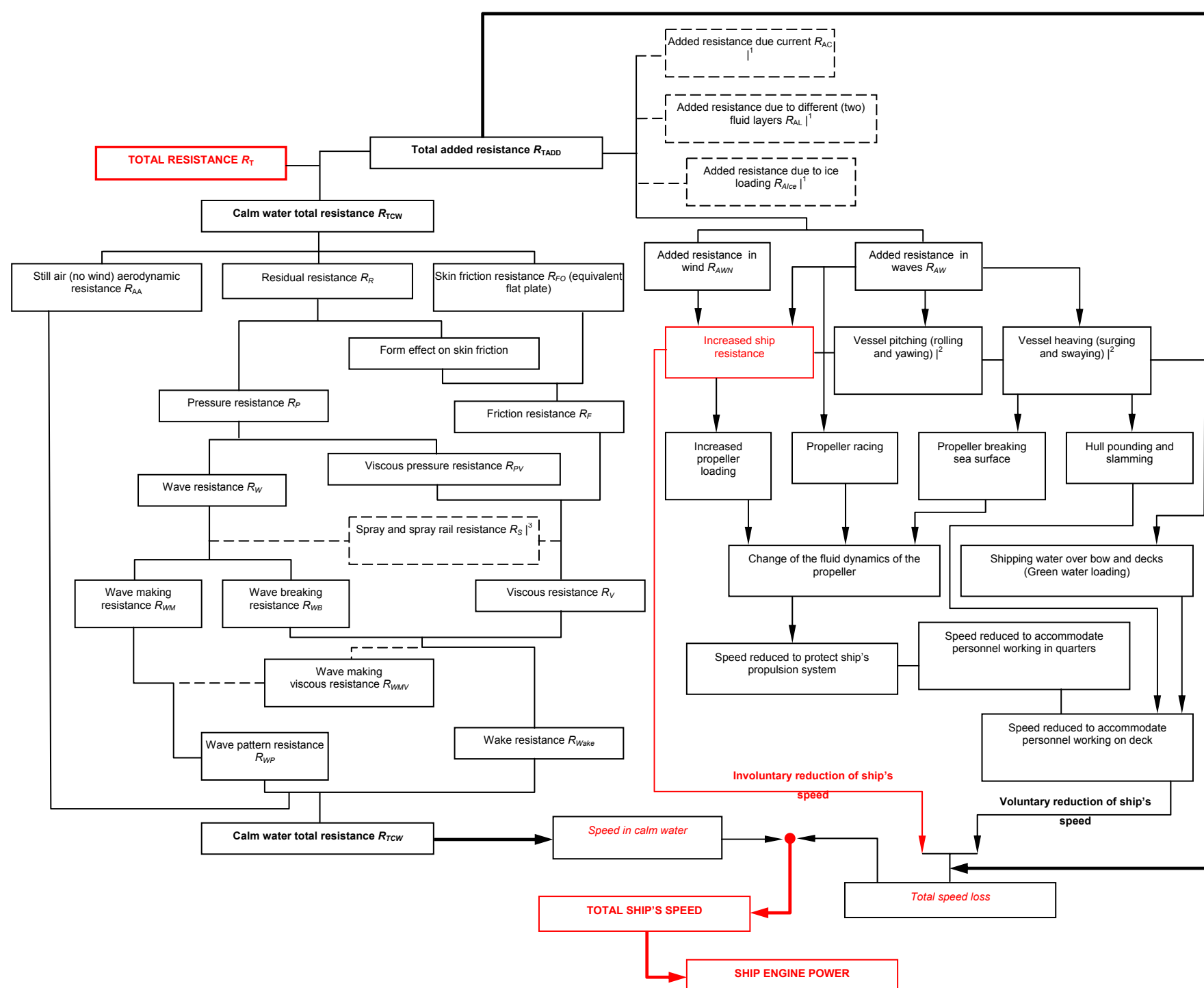
Figure A3-1 The decomposition of total resistance R_T and effects due to waves and wind loading on displacement type of ships.
