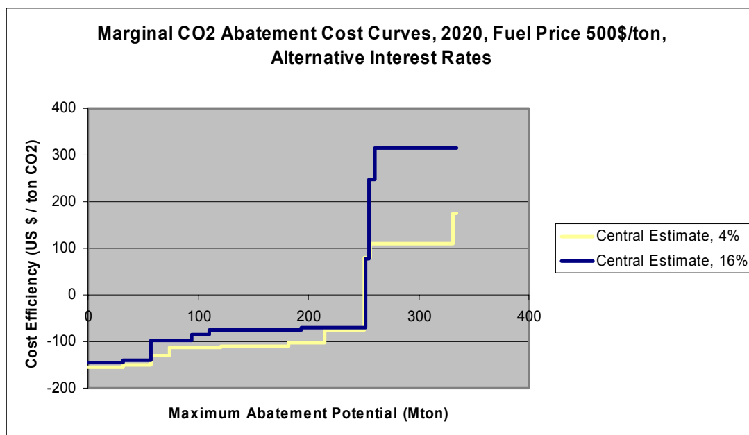
Figure A4-3 – Marginal CO 2 abatement cost curves for a fuel price of US$500/tonne and alternative interest rates, central estimate only
