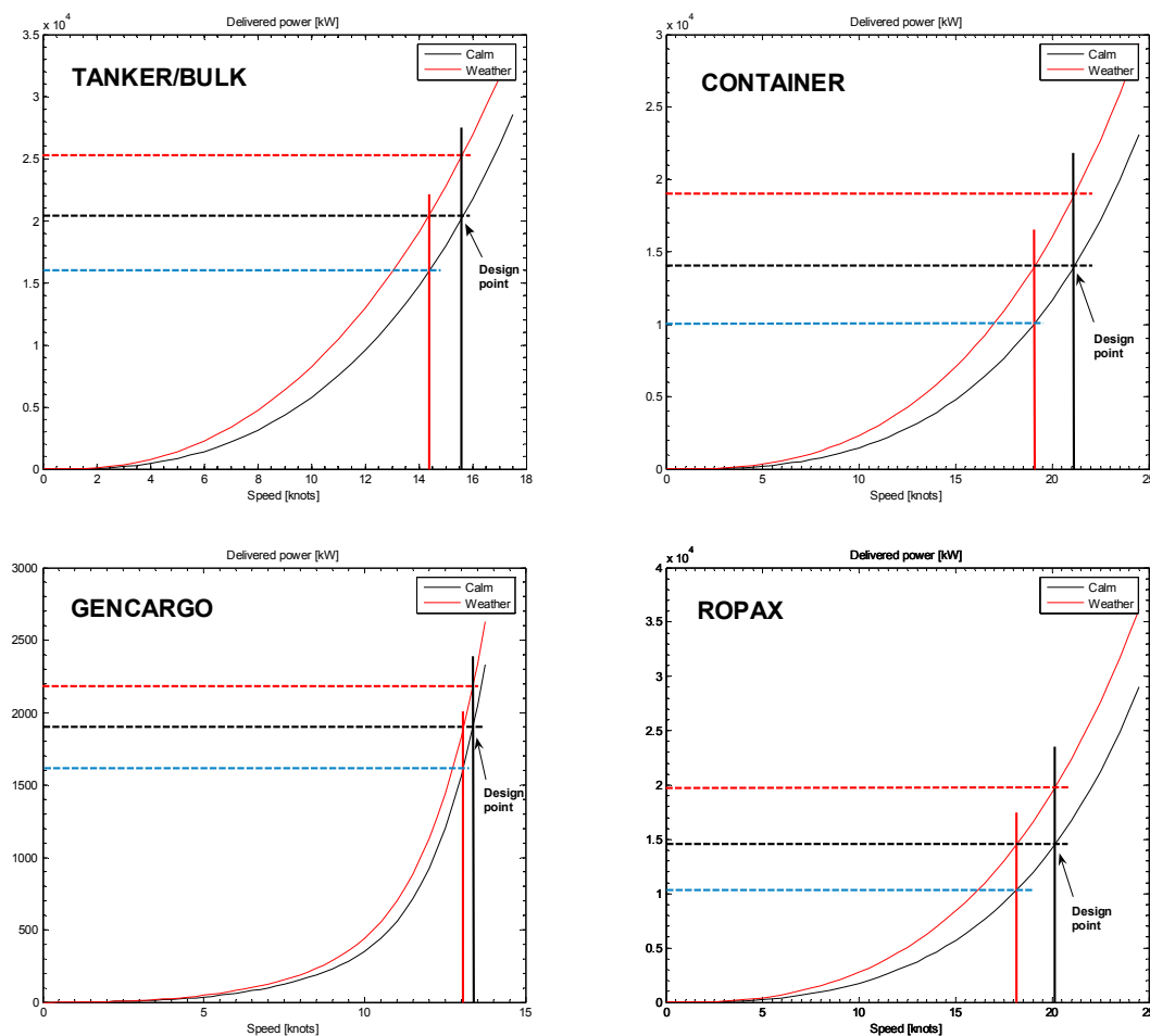
Figure A3-3 – Speed loss (drop) at constant delivered power P_D or at increased delivered power P_D , at constant speed, of the advance of vessels in head weather conditions (irregular waves and wind from the same direction 180^\circ ) for four different types of ships, according to MARINTEK’s 2008 direct model tests database, with the assumption of Beaufort number BN ( Bft ) = 6 for Tanker/Bulk, BN ( Bft ) = 6 for Container, BN ( Bft ) = 3 for GenCargo, BN ( Bft ) = 6 for RoPax
