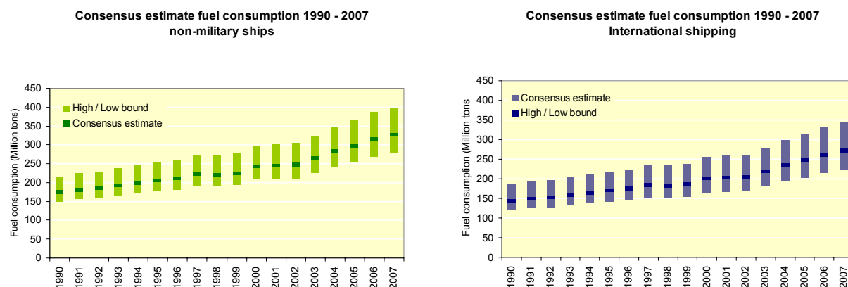
Figure A1-5 – Consensus estimates of fuel consumption from 1990 to 2007
