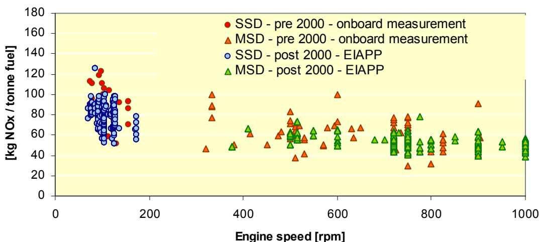
Figure 4-3 – NO x emission factors from measurement and from EIAPP certificates
