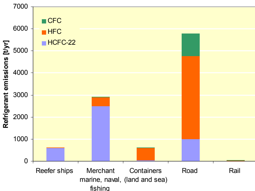
Figure 3-4 – Emissions of refrigerants from transport in 2003, UNEP [3333]
