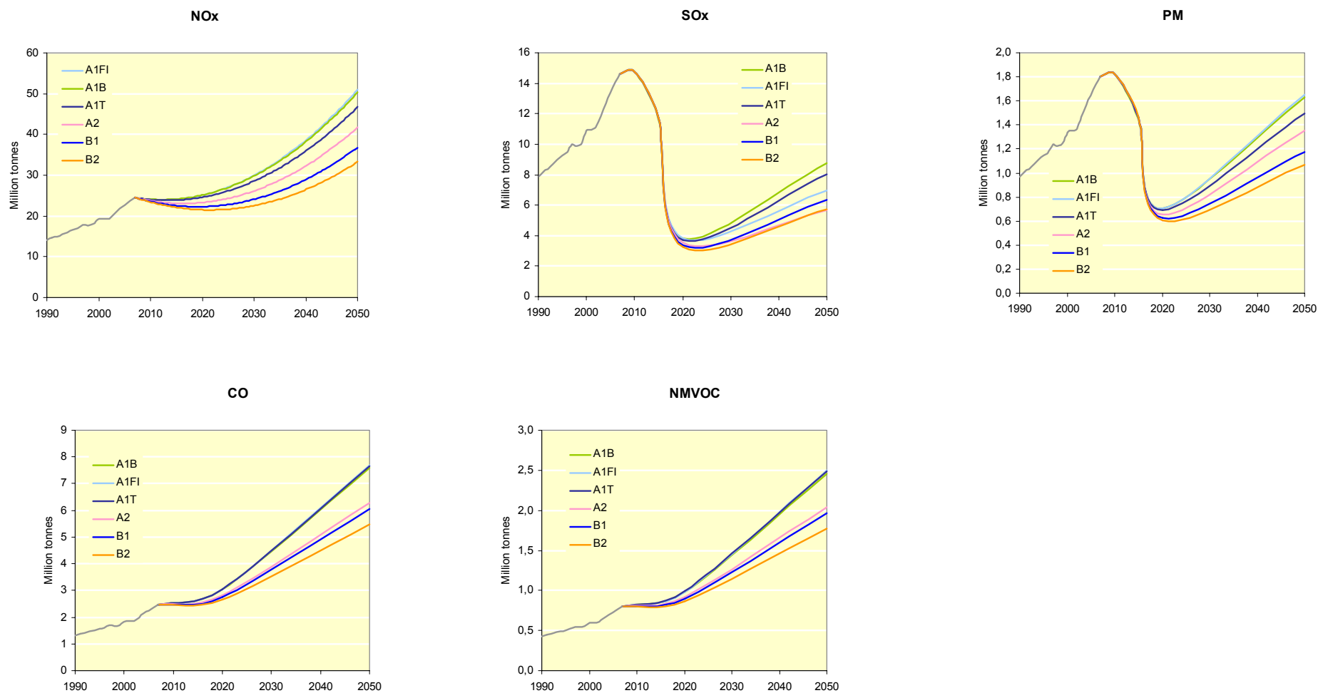
Figure 7-9 – Emission scenario trajectories for other relevant substances – total shipping (exhaust emissions only)
