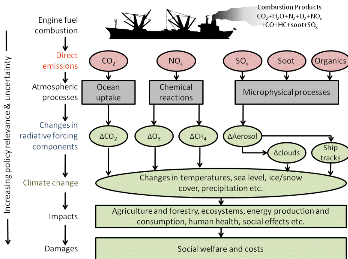
Figure 8-1 – Schematic diagram of the overall impacts of emissions for the shipping sector (from Lee et al. , 2009a)
