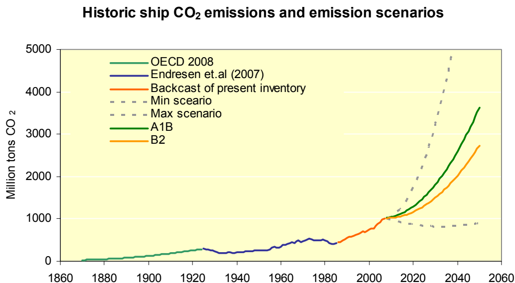
Figure 7-10 – Scenarios for emissions of CO 2 from ships in a historic perspective
