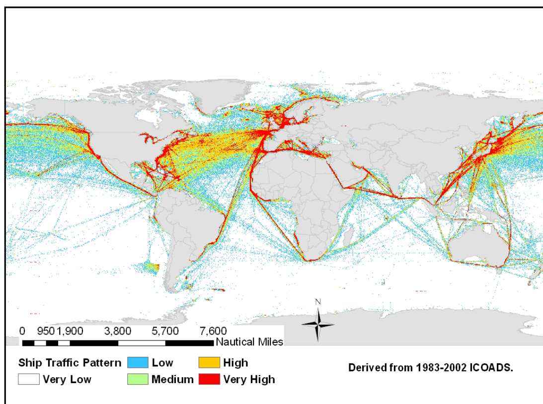
Figure A1-8 – Ship traffic patterns, based on ICOADS data
