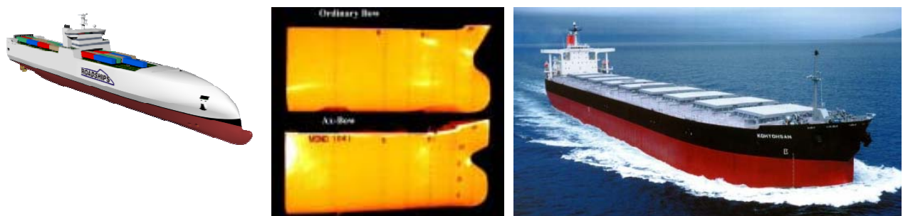
Figure A2-2 – (a) Example of a superslender monohull with outriggers (copyright STX Europe, 2008). (b) Axe-bow design and 172 000 DWT Capesize bulk carrier KOHYOHSAN, built with an axe bow for Mitsui O.S.K. Lines, Ltd in 2001.
