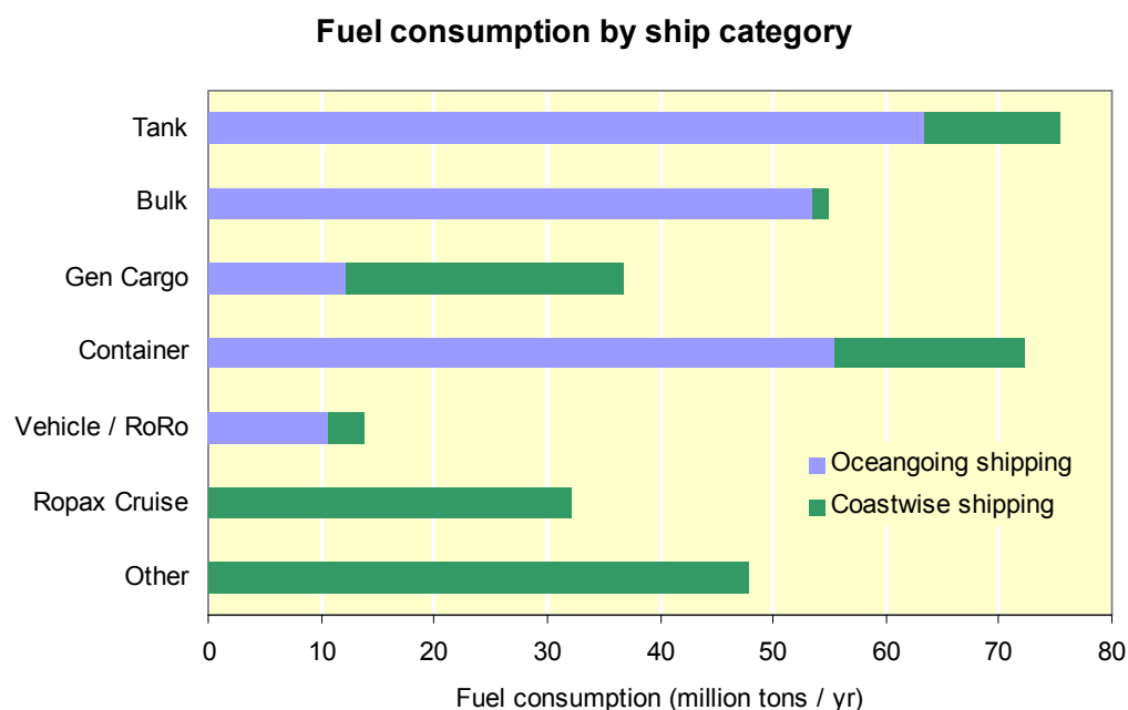
Figure A1-7 – Fuel consumption (million tonnes) by main ship categories, showing assumed typical types of operation (Coastwise shipping is mainly ships < 15000 dwt, RoPax, Cruise, Service and Fishing)
