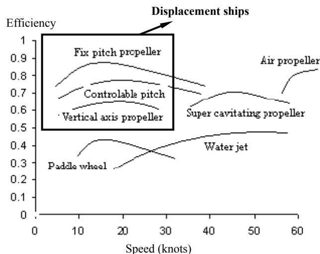
Figure A2-6 – Efficiency of propulsive devices [31]
