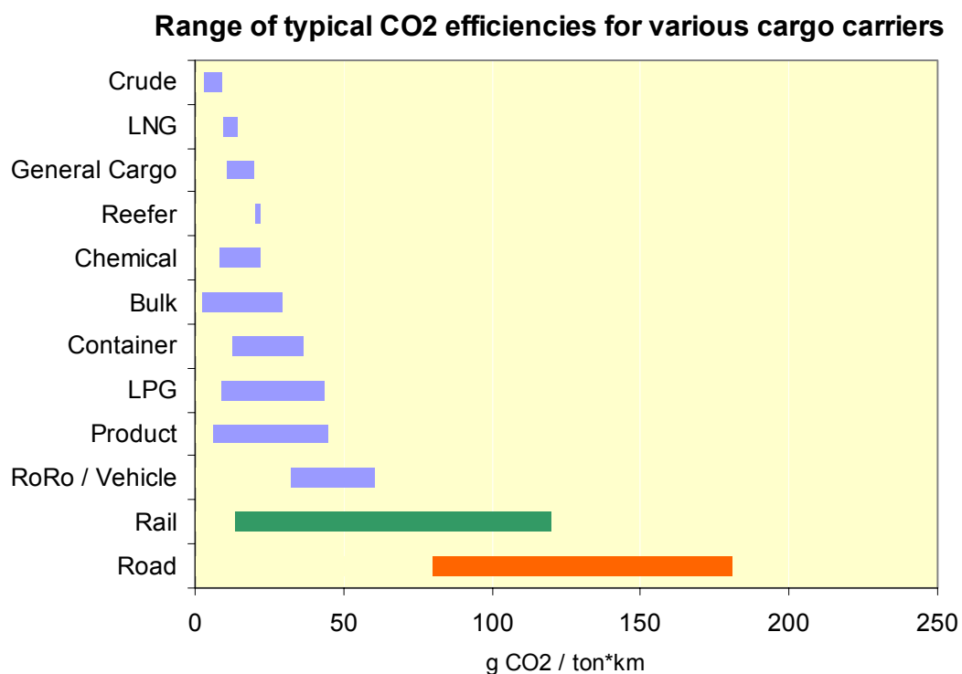
Figure 9-2 – Typical range of ship CO 2 efficiencies compared to rail and road
