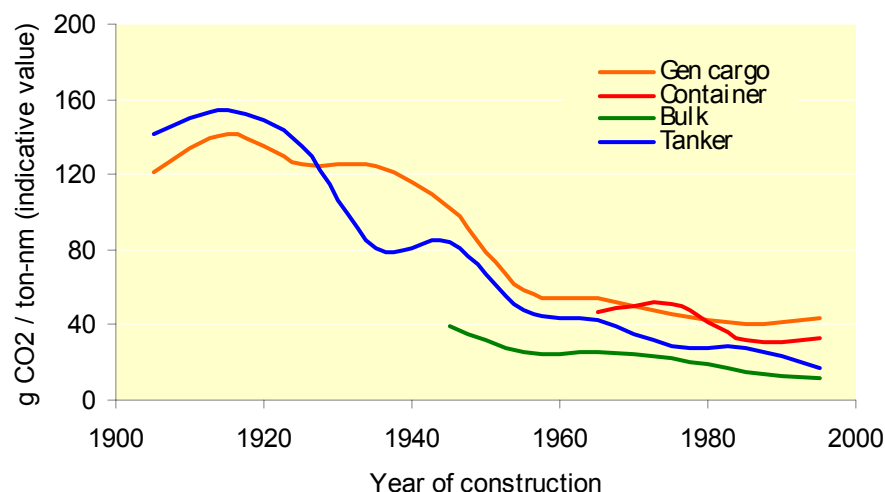
Figure 9-4 – Indicative development in average ship design transport efficiency
