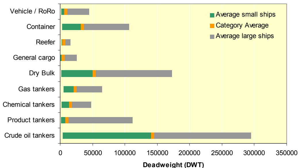
Figure 2-6 – Deadweight of major cargo ship types. High and low end represent average deadweight of the upper and lower ship size categories that were used in the study, not of individual ships, which may be significantly larger or smaller [Lloyd's Register – Fairplay, 2007]
