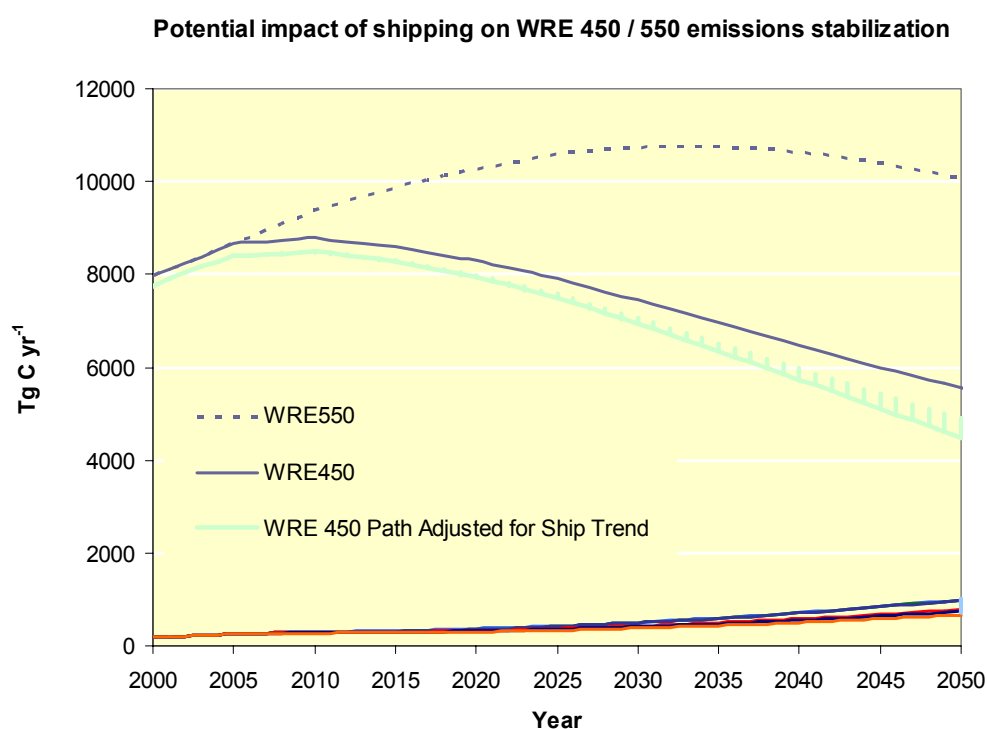
Figure 8-7 – Comparison of modelled shipping emissions, curves for WRE 450 and WRE 550, and WRE 450 adjusted for ship emissions (global total minus the emissions arising from shipping)
