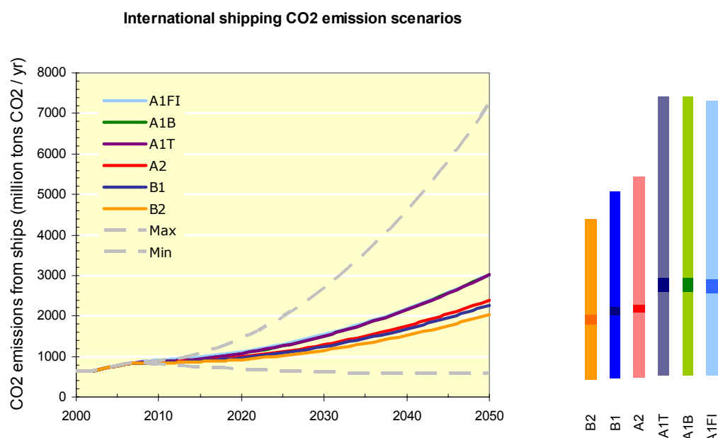
Figure7-7 – Trajectories of the emissions from international shipping. Columns on the right-hand side indicate the range of results for the scenarios within individual scenario families
