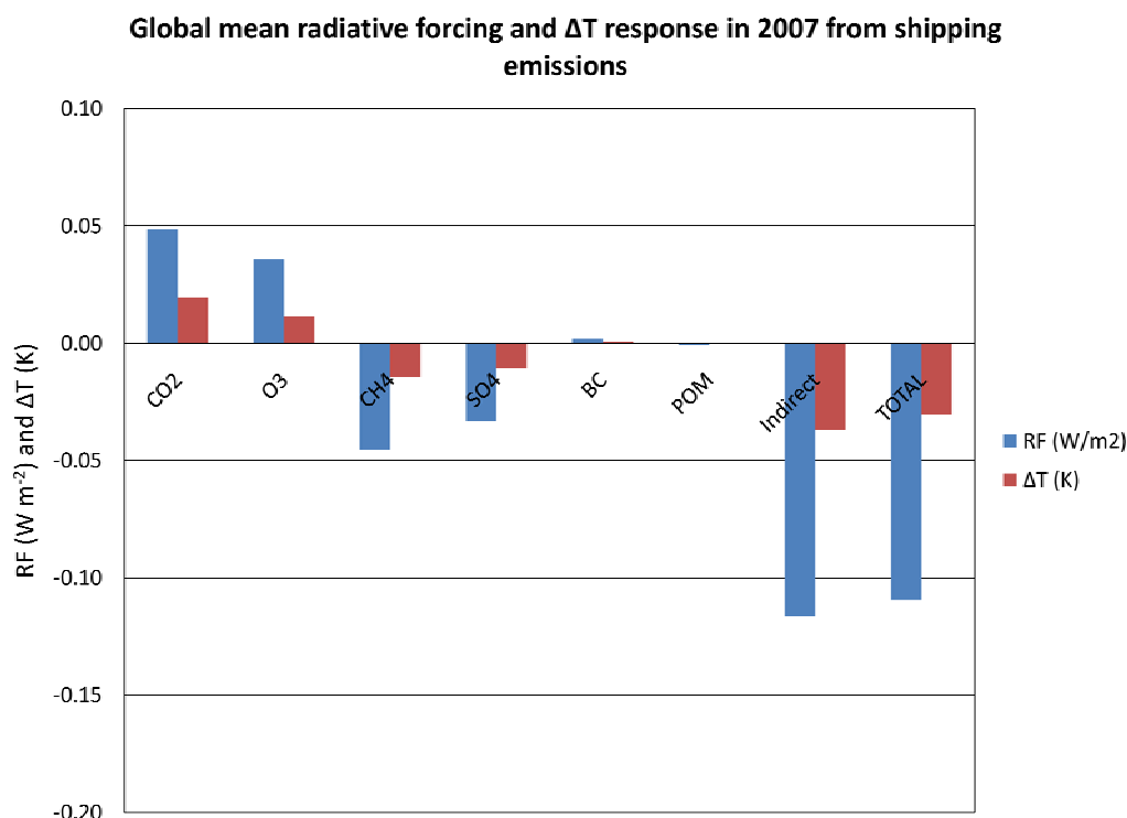
Figure 8-4 – Global mean radiative forcings ( \text{W m}^{-2} ) and temperature responses (K) in 2007 from shipping emissions. The figure does not include the positive RF that could possibly occur from the interaction of BC with snow, which has so far not been investigated for ships.
