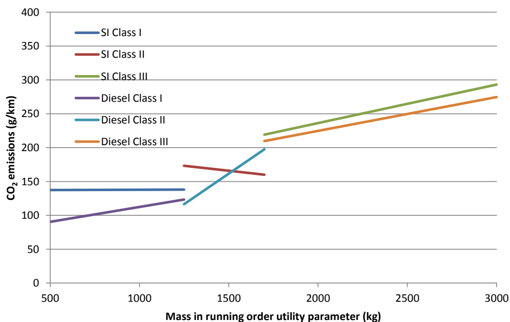
Figure 21 Sales weighted best fist of different segments
