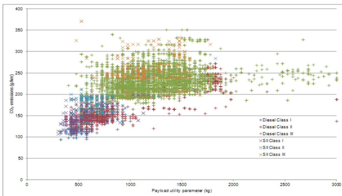
Figure 83 CO 2 and payload values of LCV sales in 2010, for the six different LCV segments
