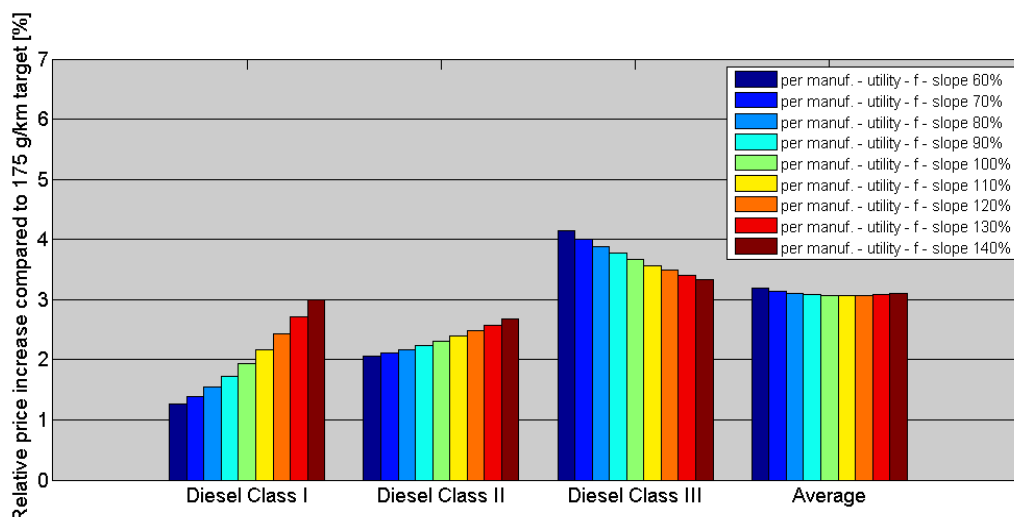
Figure 75 Relative price increase relative per segment for footprint-based limits applied per manufacturer , compared to the situation in which the 175 g/km legislation is maintained between 2017 and 2020.
