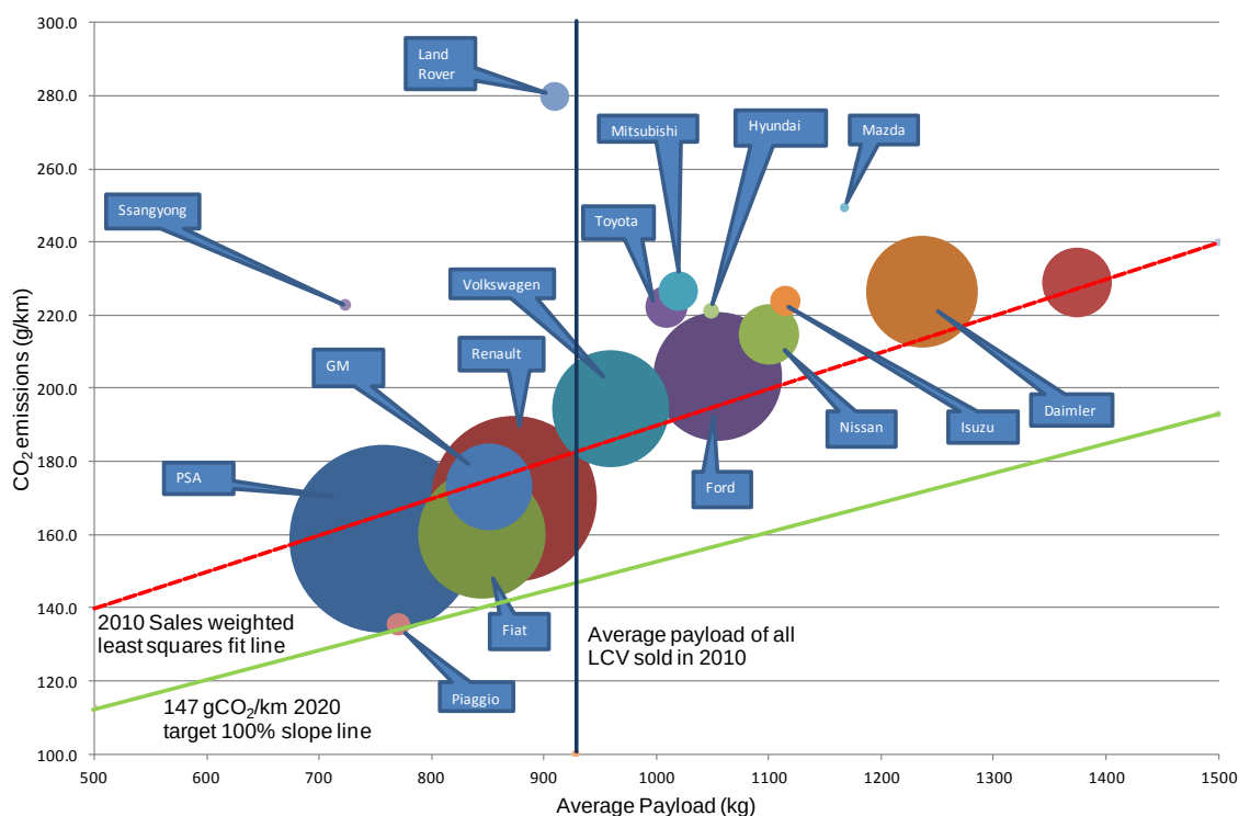
Figure 31 Average CO 2 emissions as a function of payload for various manufacturers selling LCV in Europe. The size of the bubbles indicates the sales volume.
