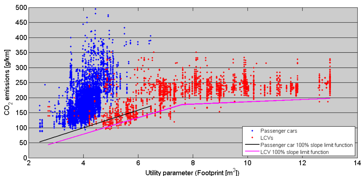
Figure 57 Comparison of 2010 LCV data and 2009 passenger car data, including the footprint based 100% slope functions for both vehicle types.
