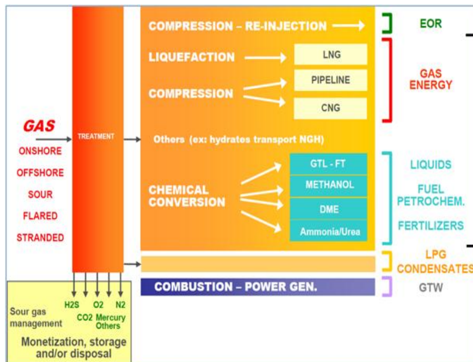
Figure 6 Potential future and existing routes for utilisation of natural gas and associated gas
