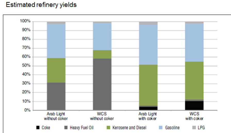
Figure 13 Yield structure dependent on refinery configuration
