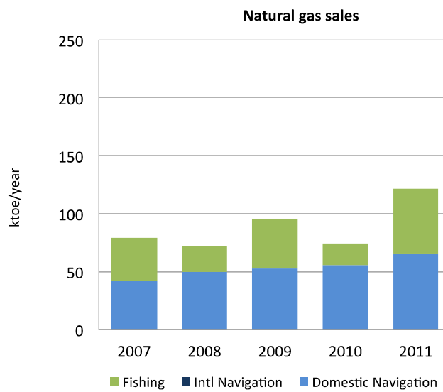
Figure 21 IEA natural gas sales in shipping 2007–2011.
