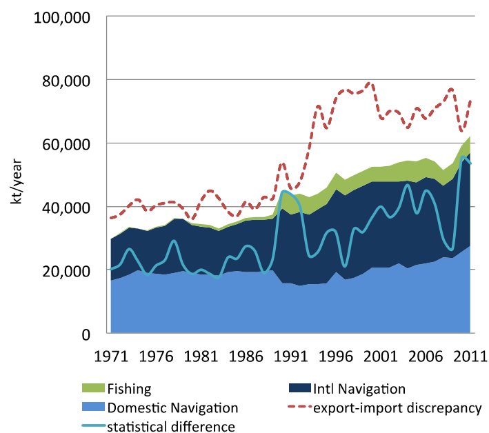
Figure 21 Gas/diesel shipping sales, export-import discrepancy and statistical difference at world balance.
