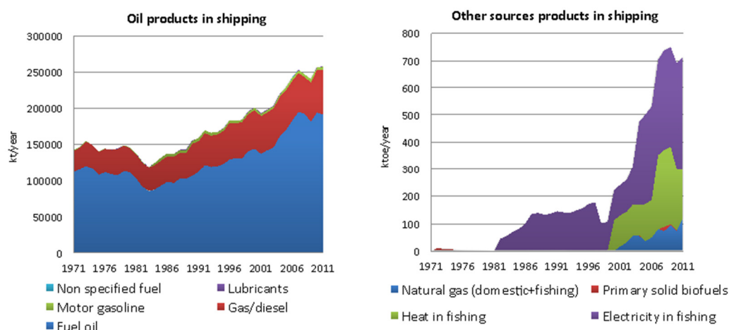
Figure 18 Oil products and products from other sources used in shipping (international, domestic and fishing) 1971–2011.
