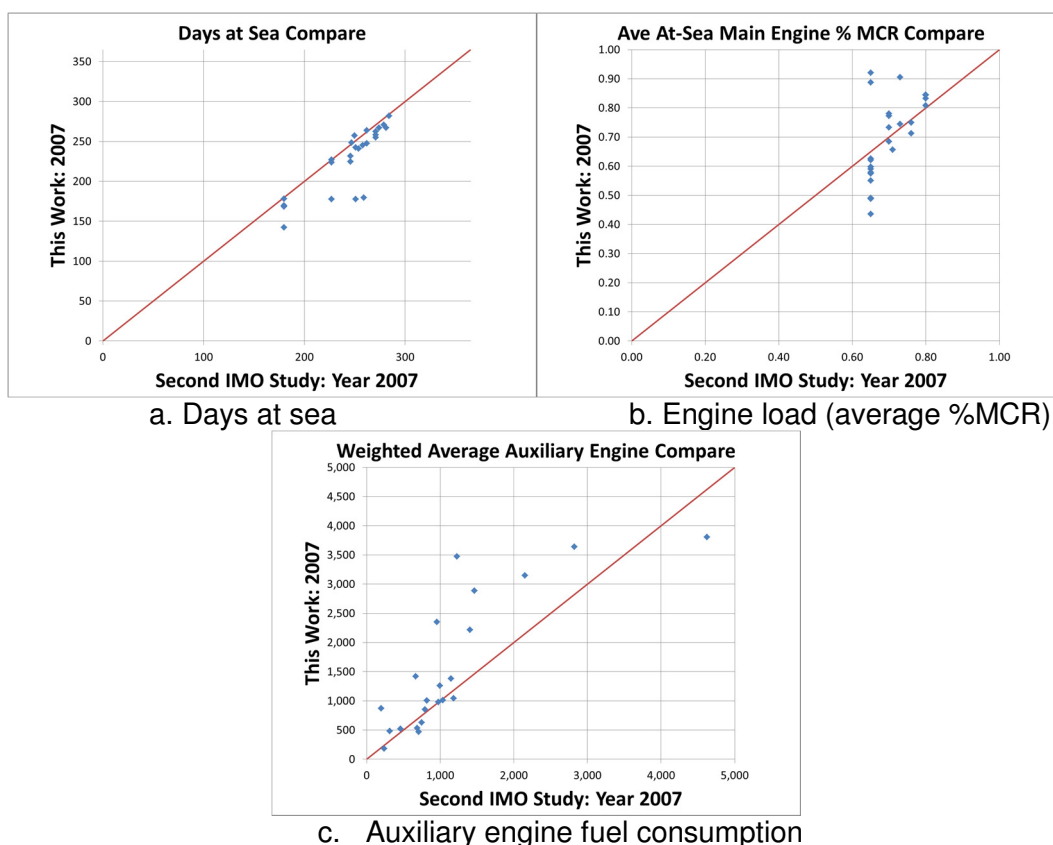
Figure 68 Crossplots for days at sea, average engine load (%MCR) and auxiliary engine fuel use for the year 2007, as reported by the IMO GHG Study 2009 (x-axis) and the IMO GHG Study 2014 (y-axis).
