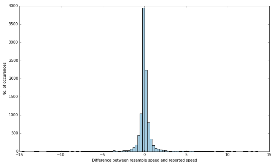
Figure 18: Distribution of difference between reported speeds when the time difference in reporting is between 2 hours (sampled as message from 105 mins to 120 mins from the original message) for all VLCC ships captured in AIS. The standard deviation of the sample was 1.85nm/hr.
