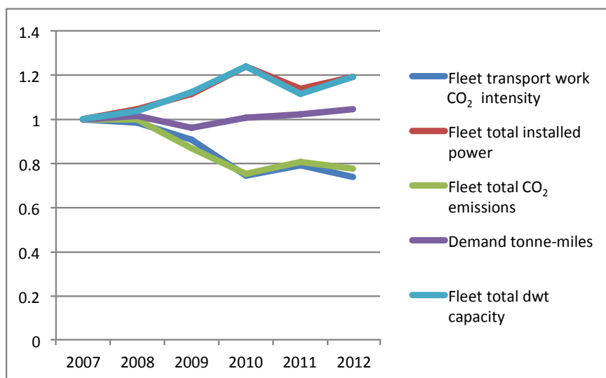
Figure 6 Time-series for trends in emissions and drivers of emissions in the oil tanker fleet 2007–2012. All trends are indexed to their values in 2007.
