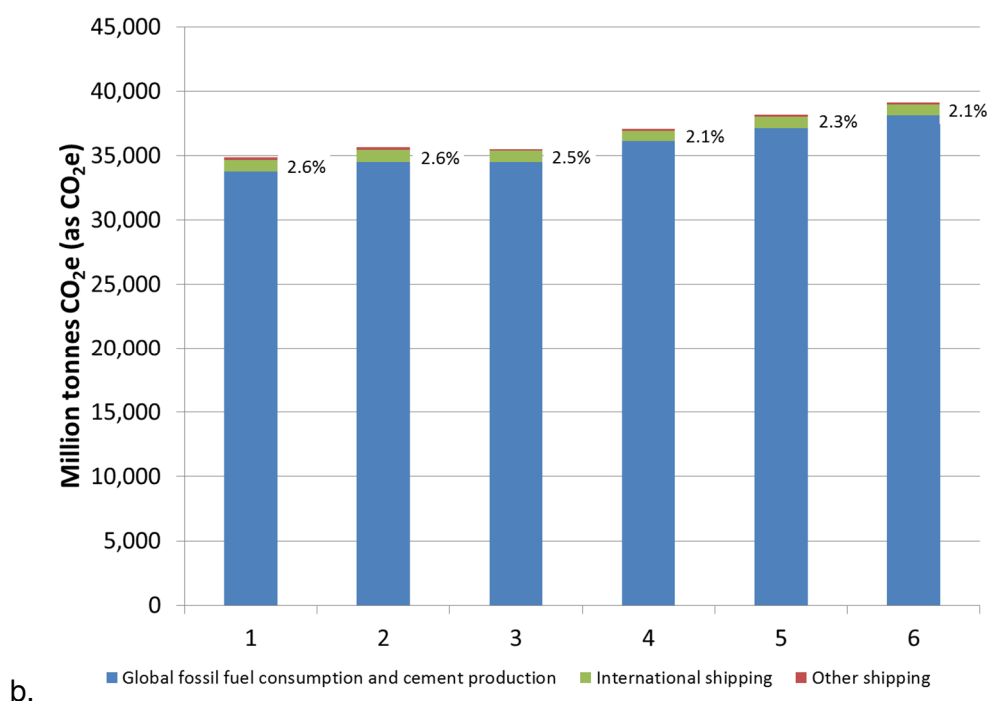
Figure 42 Comparison of shipping with global totals: a) CO 2 emissions compared, where percent shows international shipping emissions CO 2 as a percent of global CO 2 from fossil fuels; b) CO 2 e emissions compared, where percent shows international shipping emissions CO 2 e as a percent of global CO 2 e from fossil fuels.
