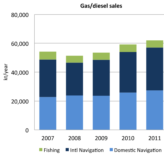
Figure 20 IEA gas/diesel sales in shipping 2007–2011.
