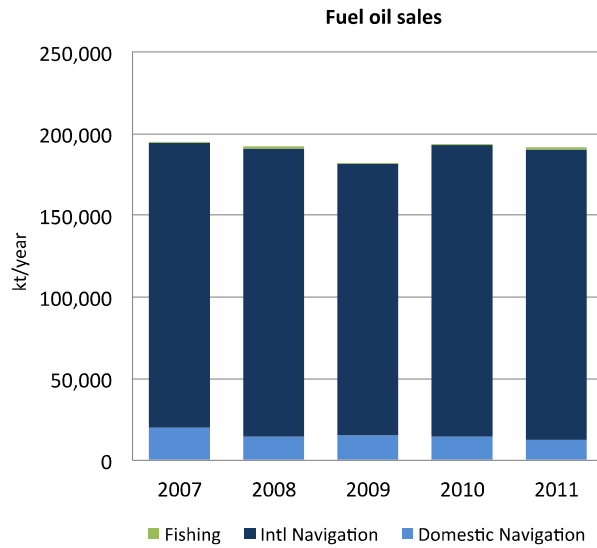
Figure 19 IEA fuel oil sales in shipping 2007–2011.
