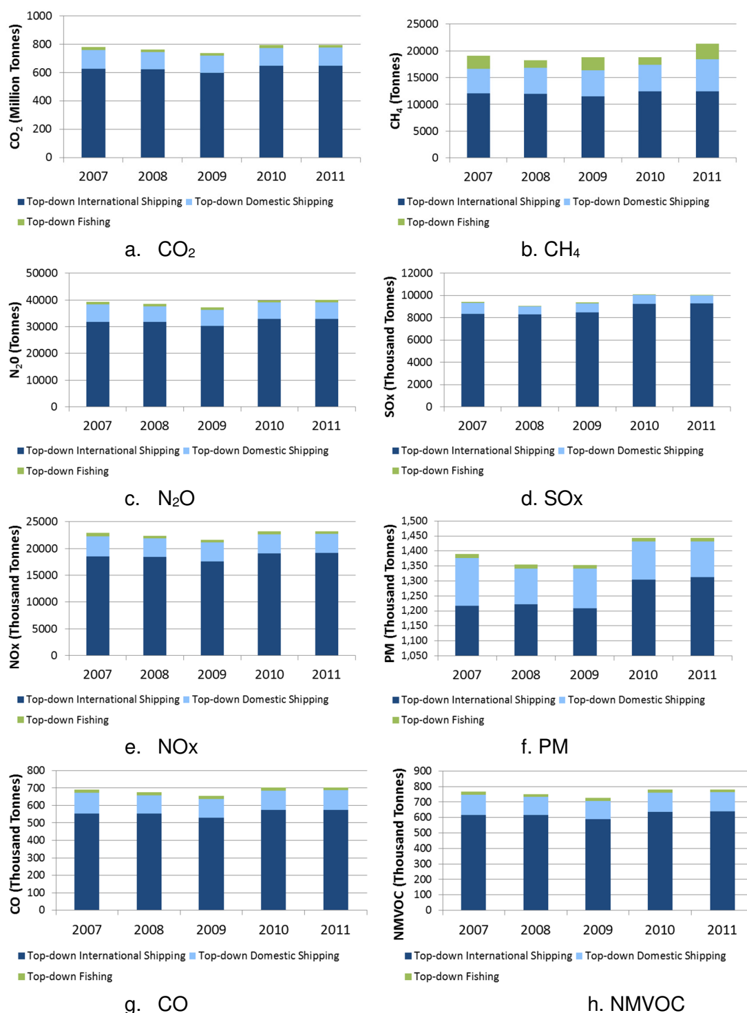
Figure 75 Time series of top-down results for a) CO 2 , b) CH 4 , c) N 2 O, d) SO x , e) NO x , f) PM, g) CO, and h) NMVOC, delineated by international shipping, domestic navigation and fishing.
