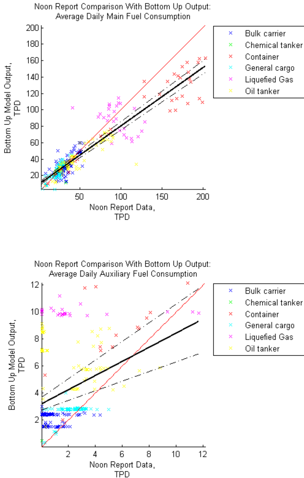
Figure 54 Average noon-reported daily fuel consumption of the main and auxiliary engine, compared with the bottom-up estimate over each quarter of 2012.
