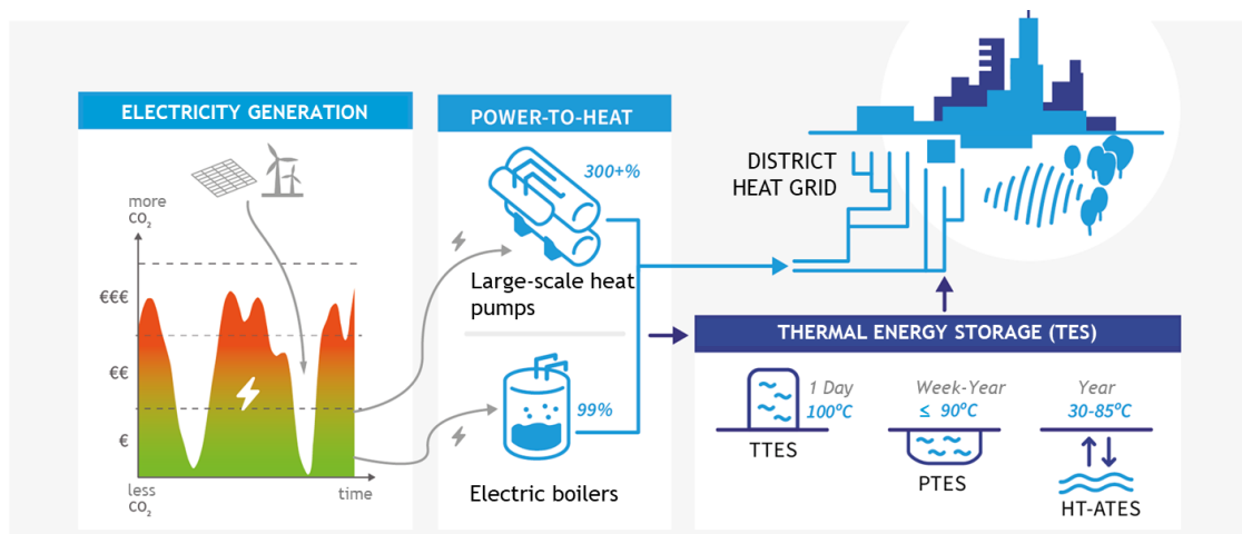
Figure 1 - Illustration of the concept of Power-to-Heat combined with thermal energy storage for heat grids
