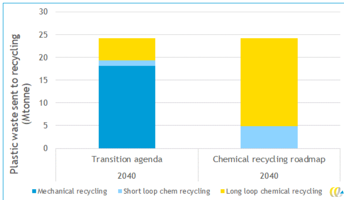
Figure 4 - Theoretical maximum available quantities of plastic waste sent to recycling (Mtonne)
